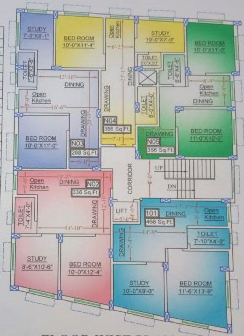
FLOOR WISE PLAN ( 1st., 2nd., 3rd. & 4th.)
